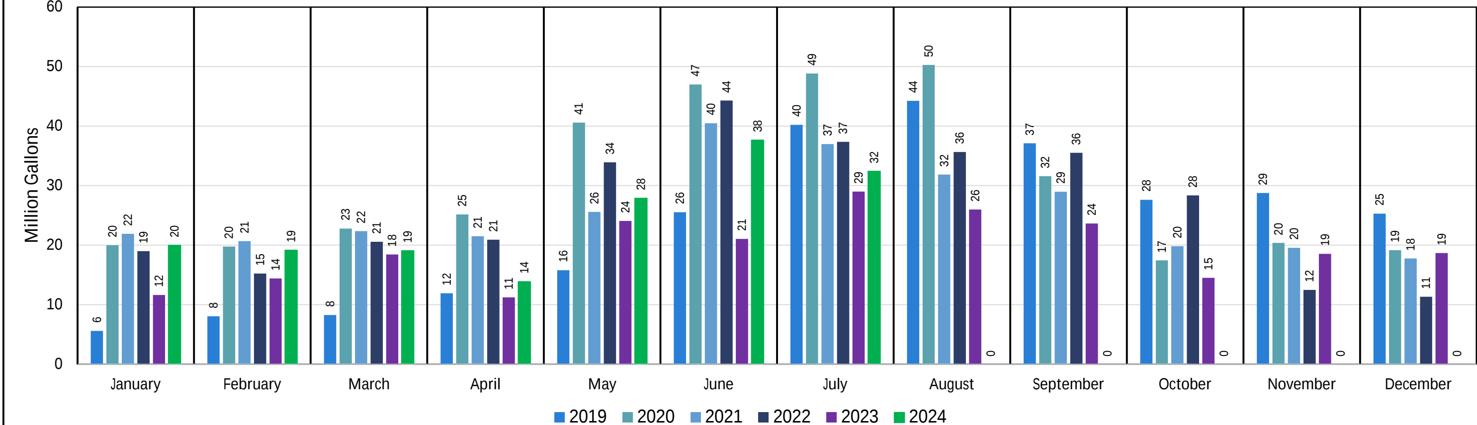
Monthly Production: Main WTP (Conventional & Microfiltration) (Through July 2024)
