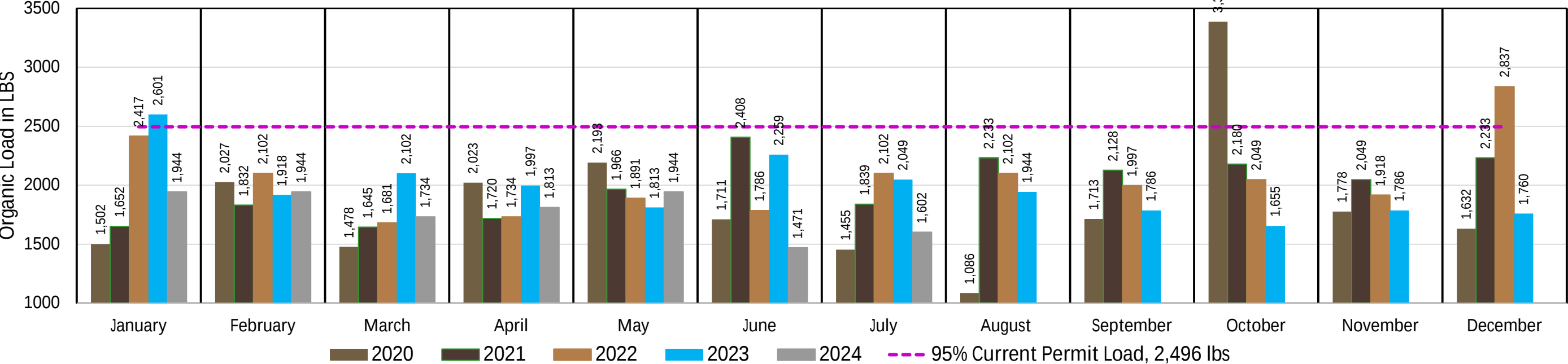
Monthly Production: Organic Loading (Through July 2024)
